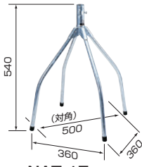
NAT-1Z
