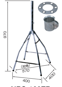
NBS-100ZR
