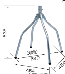
AT-5D
