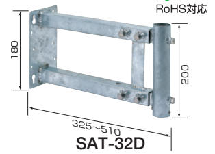
SAT-32D
